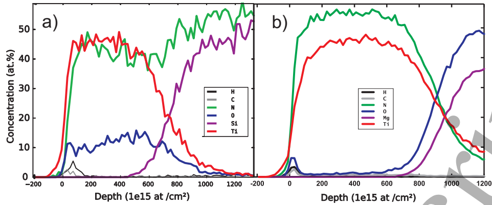
Figure 7. (a) The elemental depth profile of TiN film with the highest oxygen content, deposited on silicon nitride without chamber baking at p_N ( f_N ) = 77 mTorr (5.5 sccm). It has a T_C = 2.57 K. (b) Same for a film on MgO with chamber baking at p_N ( f_N ) = 71 mTorr (5.15 sccm). In this case T_C = 4.58 K.
