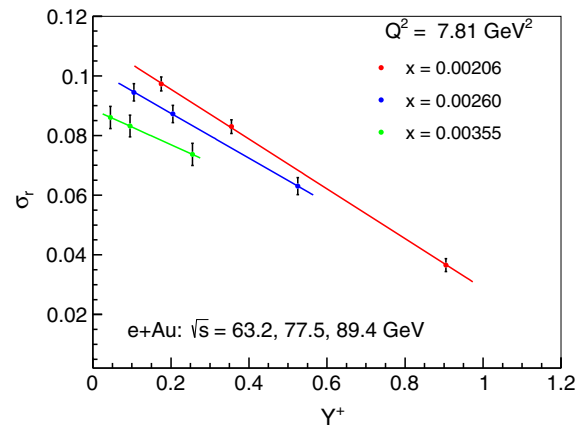
FIG. 9. The reduced cross section for e + \text{Au} collisions at \sqrt{s} = 63.2, 77.5 and 89.4 GeV versus Y^+ for Q^2 = 7.81 GeV 2 for three values of x . Fitting the slope of each data set with fixed x gives the negative of F_L .
