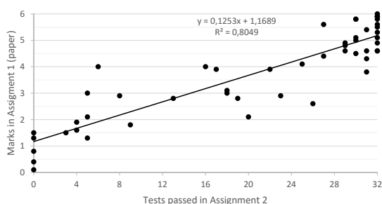
Figure 5: The number of passed tests in Assignment 2 (automatic assessment) compared to Assignment 1 marks (manual assessment).
