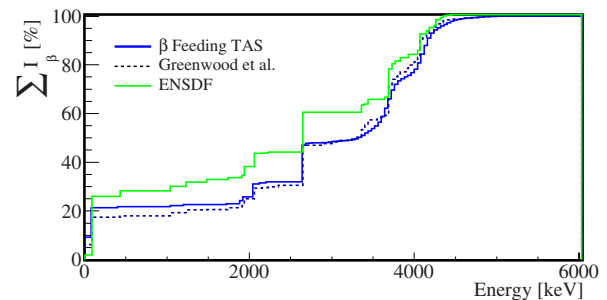
Figure 4. Accumulated feeding distribution from the analysis of the ^{91}\text{Rb} decay compared with the feeding distribution available in ENSDF and with the obtained by Greenwood et al. [7].
