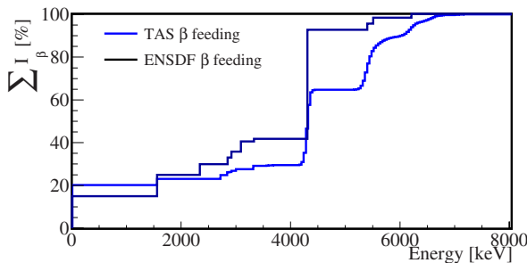
Figure 2. Accumulated feeding distribution from the analysis of the ^{86}\text{Br} decay compared with the feeding distribution available in ENSDF.
