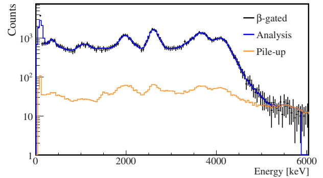
Figure 3. Comparison of the beta gated ^{91}\text{Rb} decay TAS spectrum with the spectrum generated after the analysis. The contribution of the contaminants is also presented in the figure.
