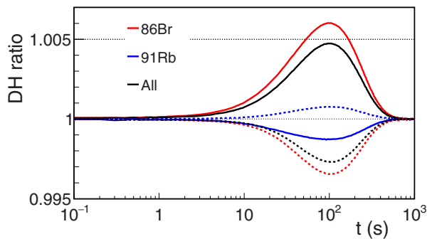
Figure 6. Relative contribution to the gamma and beta components of the decay heat of the presented decays ( ^{86}\text{Br} and ^{91}\text{Rb} ) compared with the high-resolution contribution for ^{235}\text{U} . The gamma component is represented by the continuous line. The beta component is showed with the dotted line.
