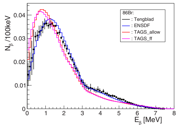
Figure 5. Comparison of the beta spectrum of the decay of ^{86}\text{Br} measured by Tengblad et al. [25] with the beta spectrum deduced from the TAS measurements. The effect of considering all beta transitions allowed or first forbidden in the deduction of the beta spectrum from the TAS measurements is also presented.
