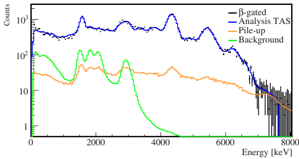
Figure 1. Comparison of the beta gated ^{86}\text{Br} decay TAS spectrum with the spectrum generated after the analysis. The contribution of the contaminants is also presented.
