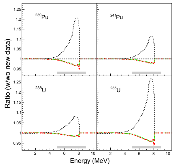
Figure 2. Ratio between the antineutrino spectra calculated using the latest TAGS results with respect to the data on ^{92}\text{Rb} decay used in [4] (thick red dashed-dotted line), in [20] (green dotted line) and in [17] (black dashed line). The sharp drop in the ratio, in one single bin located at the Q value of the ^{92}\text{Rb} , is due to the different values in Q given in [27] and ENSDF , that were used to reconstruct the antineutrino spectrum.
