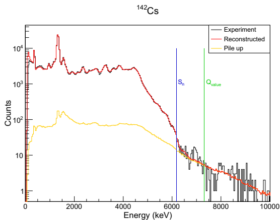
Figure 3. ^{142}\text{Cs} : comparison between measured spectrum (black continuous line) and reconstructed one (red continuous line) with the feeding obtained from the TAGS data analysis. The contribution of pile-up signals is shown (yellow line).
