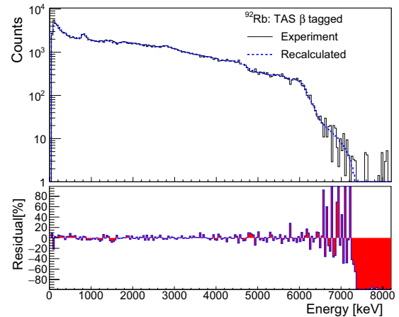
Figure 1. Upper panel: comparison between measured spectrum (black continuous line) and reconstructed one (blue dashed line) with the feeding obtained from the TAGS data analysis. Lower panel: residues between the two curves reported in the upper panel.
