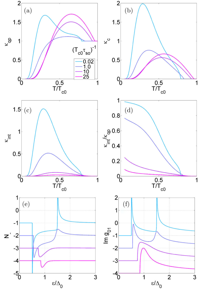
FIG. 2. Temperature dependencies of heat conductance contributions (a) \kappa_{qp} , (c) \kappa_{\text{int}} , and their ratio (d) \kappa_{\text{int}}/\kappa_{qp} for the SFS structure shown in Fig. 1 with \mathbf{h}_{1,2} \perp \mathbf{m} and the 100% spin filtering P = 1 . (b) \kappa_c for the same structure but with P = 0.8 and \theta_h = \pi/4 . Note that the quantities \kappa_{qp} , \kappa_c , and \kappa_s defined by Eqs. (9), (10), and (10) are dimensionless. (e) Total DOS N_+(\varepsilon) and (f) spin-singlet anomalous function \text{Im} g_{01}(\varepsilon) . The exchange field is h = 0.5\Delta_0 and the values of spin relaxation rate (T_{c0}\tau_{so})^{-1} shown in (a) are the same for all panels.
