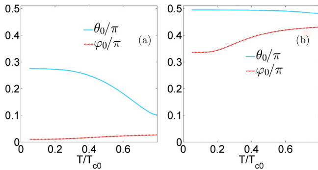
FIG. 3. The phase shifts of CPR \varphi_0 = \varphi_0(T) and HCPR \theta_0 = \theta_0(T) for (a) P = 0.8 ( r = 0.6 ) and (b) P = 0.9999 ( r = 0.014 ). Exchange splitting h = 0.5\Delta_0 and SO relaxation (T_{c0}\tau_{so})^{-1} = 1 . The magnetic configuration is that \mathbf{h}_{1,2} \perp \mathbf{m} and \theta_h = \pi/2 .
