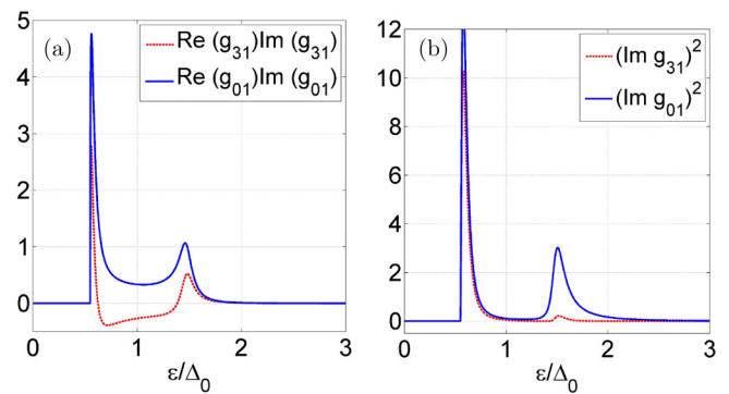
FIG. 4. Spectral amplitudes of the different components of (a) Josephson charge currents (12),(13) and (b) heat currents (10),(11). The blue solid lines and red dashed lines correspond to the contributions of spin-singlet and spin-triplet Cooper pairs, respectively. Exchange splitting h = 0.5\Delta_0 , temperature T = 0.1T_{c0} , and SO relaxation (T_{c0}\tau_{so})^{-1} = 1 .
