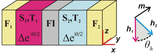
FIG. 1. The sketch of an FS-FI-SF system under the thermal bias with the superconducting electrodes S_{1,2} residing at different temperatures T_{1,2} . The exchange fields \mathbf{h}_1 and \mathbf{h}_2 in ferromagnetic electrodes F_1 and F_2 form a noncoplanar system with the spin polarization \mathbf{m} of the ferromagnetic barrier (FI).
