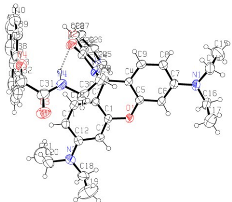
Fig. 1: ORTEP diagram of probe NpRD . Ellipsoids are drawn at 50% probability level.
