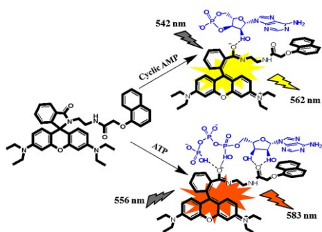
Scheme 1: Fluorescence changing of NpRD on addition of cAMP and ATP
