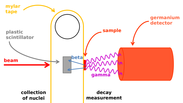
Figure 1. The experimental set-up consisted of a tape for collection and transport of the radioactive samples, a plastic scintillator to detect \beta particles, and a germanium detector for \gamma rays. The sample transport was about 12 cm. The distance between the sample once transported to the measurement position and the entrance window of the germanium detector was 15 cm. Figure not to scale.
