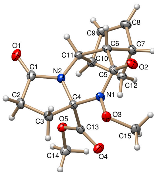
Figure 2. ORTEP plot of the X-ray structure of (±)- 4b .
