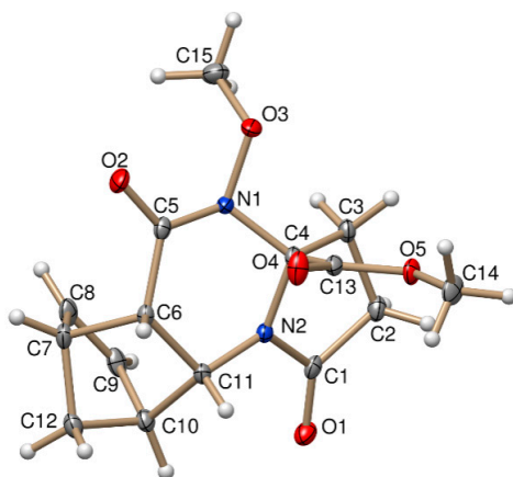
Figure 1. Oak Ridge Thermal Ellipsoid Plot (ORTEP) plot of the X-ray structure of (±)- 3a .
