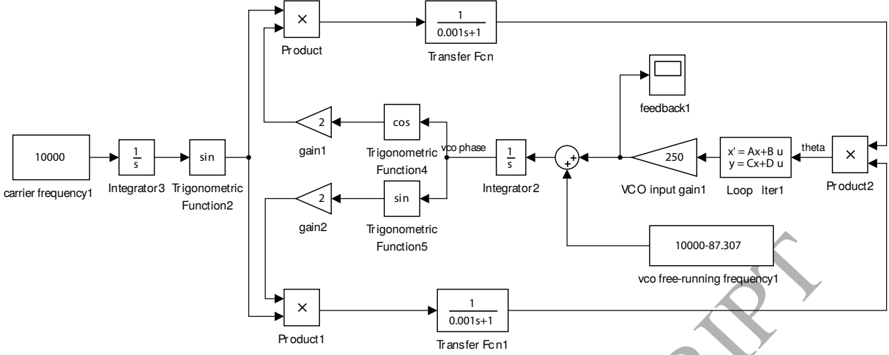
Figure 12: MATLAB Simulink model of BPSK Costas loop in the signal space ( A \rightarrow A, b \rightarrow B, c \rightarrow C, h \rightarrow D; \omega_e^{\text{free}} = 87.307 , VCO input gain is K_{\text{vco}} = 250 , \omega_{\text{ref}} = 10000 , a = 1000 )
