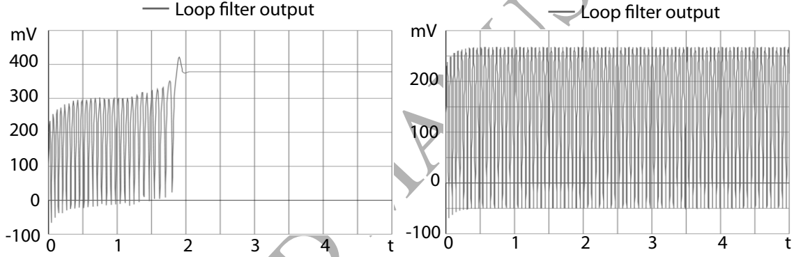
Figure 7: Simulation of the two-phase PLL in NGSPICE. For default simulation step (10m) the VCO synchronizes to the reference signal (left subfigure). For simulation step 1m an undamped oscillation exists (right subfigure). Parameters: K_{vco} = 250 , A = -15.7978 , b = 0.7077 , c = 15.7978 , h = 0.2923 ( \tau_1 = 0.0448 , \tau_2 = 0.0185 ), \omega_e^{free} = 189 . Initial charge of capacitor C2 is 50m (corresponds to initial state of the Loop filter), \theta_e(0) = 0 , \omega_{ref} = 10000 .
