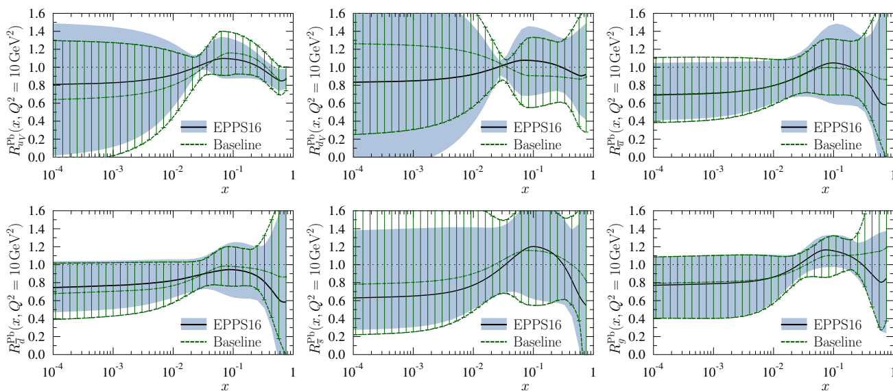
Fig. 22 The nuclear modifications at Q^2 = 10 \text{ GeV}^2 from the EPPS16 fit (black central line and light-blue bands) compared with the baseline fit (green curves with hatching) which uses only the data included in the EPS09 fit
