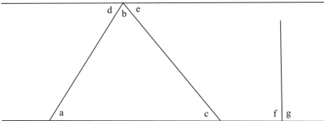
Figure 1. Demonstration that the sum of the angles of an Euclidian triangle equals two right angles.
