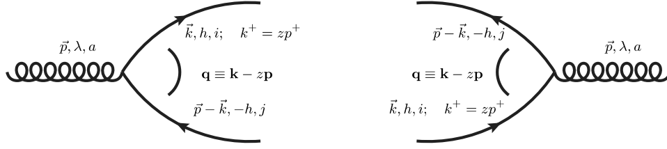
FIG. 2: Left: Gluon splitting vertex into quark-antiquark pair, A_{\lambda,h}^{a;ij}(\mathbf{q}, z) Eq. (17). Right: Quark-antiquark annihilation vertex into gluon A_{\lambda,h}^{i;ja}(\mathbf{q}, z) Eq. (18).
