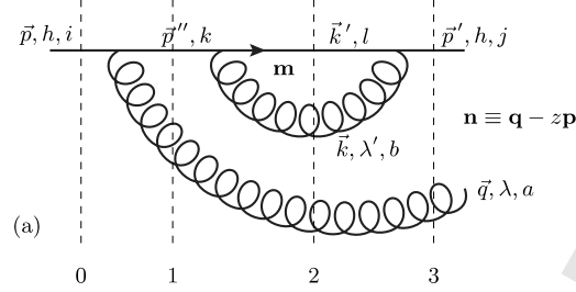
FIG. 8: Contribution to gluon emission from final state quark propagator correction, diagram (a), with energy denominator intermediate states and kinematics. Momentum conservation: \vec{p} = \vec{p}' + \vec{q} and \vec{p}' = \vec{k}' + \vec{k} . The momentum fraction and natural momentum scale for the emitted gluon are z = q^+ / p^+ and \mathbf{n} = \mathbf{q} - z\mathbf{p} . The momentum fraction for the gluon in the loop is z' = k^+ / p^+ , i.e. k^+ = z'(1-z)p^+ and the natural momentum \mathbf{m} = \mathbf{k} - z'\mathbf{p}' .
