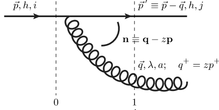
FIG. 7: Gluon emission at leading order. Momentum is conserved \vec{p} = \vec{p}' + \vec{q} , and the momentum fraction and natural transverse momentum for the emitted gluon are z = q^+ / p^+ and \mathbf{n} = \mathbf{q} - z\mathbf{p} .
