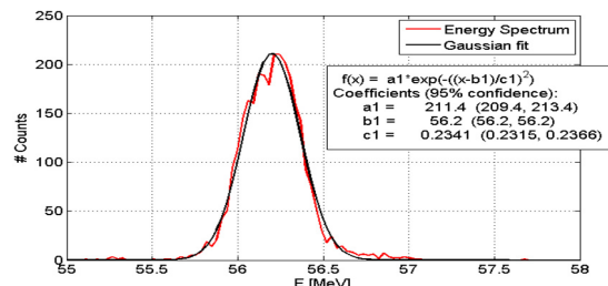
Figure 3: Energy spectrum of a pilot ^{14}\text{N}^{4+} beam used to set up the accelerator before ^{76}\text{Zn}^{22+} and ^{74}\text{Zn}^{21+} were delivered to the users ( E = 4.0 \text{ MeV/u} , \Delta E_{\text{FWHM}} \lesssim 0.7 \% ).
