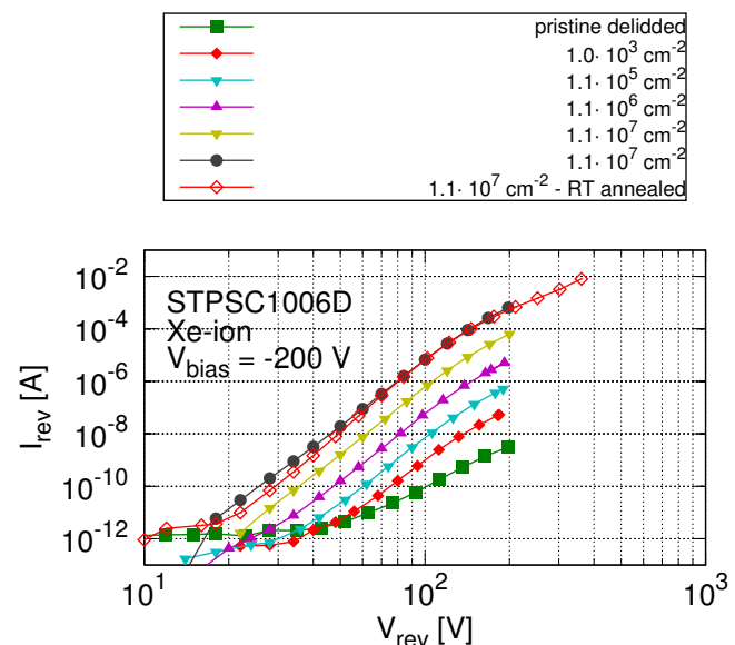
Figure 2. Reverse current-voltage characteristics for a STPSC1006D diode before and after exposure to Xe ions at a bias of -200\text{V} . Room temperature (RT) annealed data was taken 3 months after the heavy-ion exposure.
