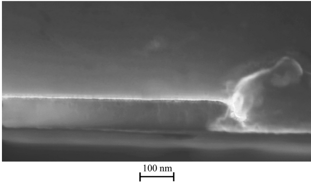
FIG. 2. PEALD AlN film of 100 nm thickness on silicon after patterning (etched region) in a caustic solution.
