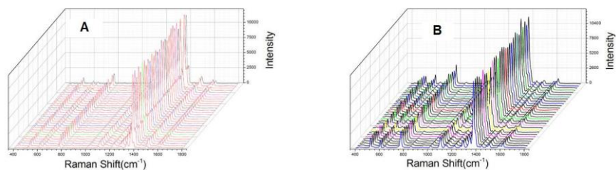
Fig. 3. Raman Spectra of SERS mapping in two different regions (10 \mu m x 10 \mu m, step size of 2 \mu m) obtained from vertical 3D nanorod supercrystal.
