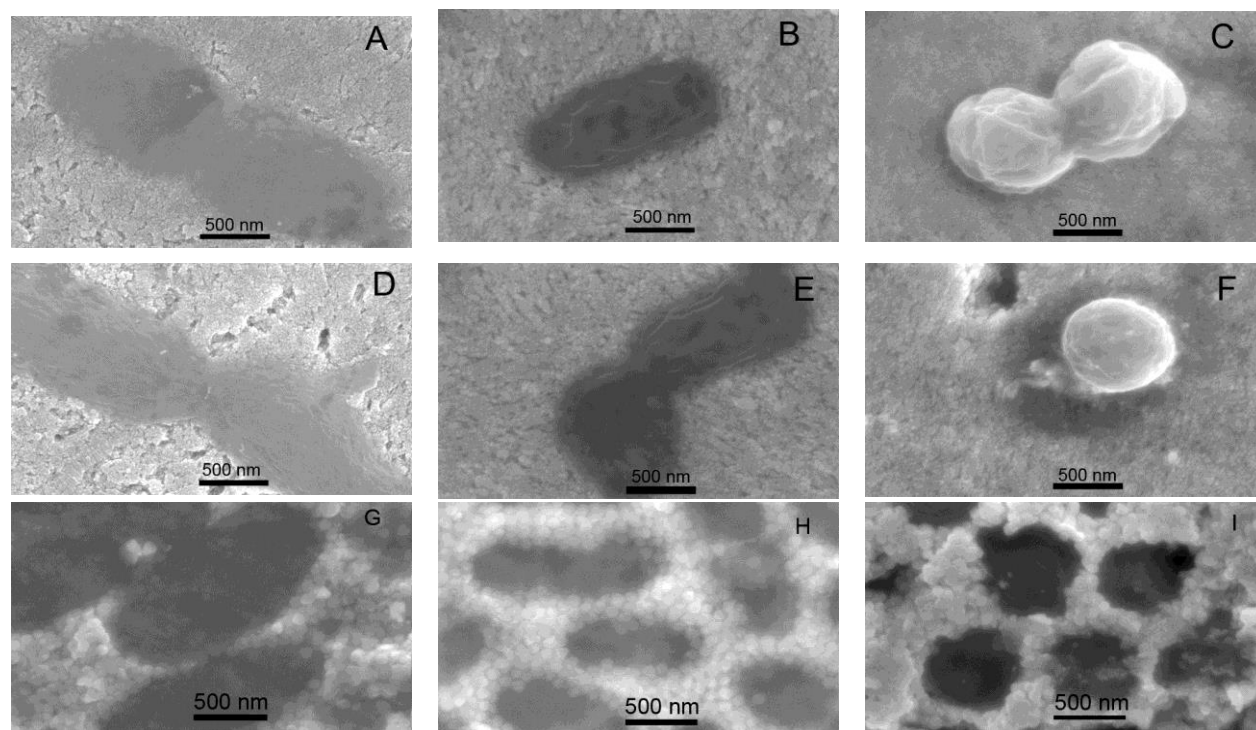
Fig. 2. SEM images of A: E. coli on a 3D vertical supercrystal of plasmonic nanorods; B: S. enterica on a 3D vertical supercrystal of plasmonic nanorods; C: S. xylosus on a 3D vertical supercrystal of plasmonic nanorods; D: E. coli on a vancomycin-coated 3D vertical supercrystal of plasmonic nanorods; E: S. enterica on a vancomycin-coated 3D vertical supercrystal of plasmonic nanorods; F: S. xylosus on a vancomycin-coated 3D vertical supercrystal of plasmonic nanorods; G: plasmonic 3D nanoplate aggregate- E. coli -vertical nanorod supercrystal; H: plasmonic 3D nanoplate aggregate- S. enterica -vertical nanorod supercrystal; I: plasmonic 3D nanoplates aggregate- S. xylosus -vertical nanorod supercrystal.
