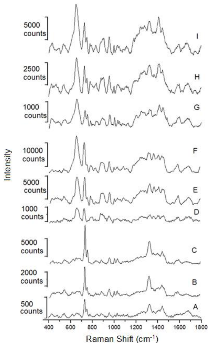
Fig. 6. SERS spectra of A: S. xylosus on a plasmonic vertical nanorod supercrystal, B: S. xylosus on a vancomycin-coated plasmonic vertical nanorod supercrystal, C: S. xylosus embedded in a plasmonic nanoplate aggregate/vertical nanorod supercrystal, D: S. enterica on a plasmonic vertical nanorod supercrystal, E: S. enterica on a vancomycin-coated plasmonic vertical nanorod supercrystal, F: S. enterica embedded in a plasmonic nanoplate aggregate/vertical nanorod supercrystal, G: E. coli on a plasmonic vertical nanorod supercrystal, H: E. coli on a vancomycin-coated plasmonic vertical nanorod supercrystal, I: E. coli embedded in a plasmonic nanoplate aggregate/vertical nanorod supercrystal.
