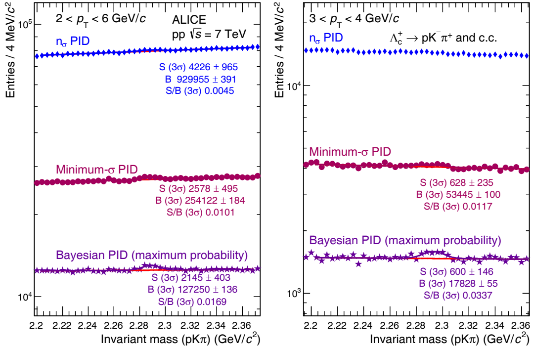
Fig. 15. Invariant mass spectra of \Lambda_c^+ \rightarrow pK^- \pi^+ using n_\sigma PID, minimum- \sigma PID and Bayesian PID for (left) 2 < p_T < 6 \text{ GeV}/c and (right) 3 < p_T < 4 \text{ GeV}/c . Due to the low statistical significance, it was not possible to extract a stable signal for n_\sigma PID for 3 < p_T < 4 \text{ GeV}/c , therefore this fit and its results are not shown.
