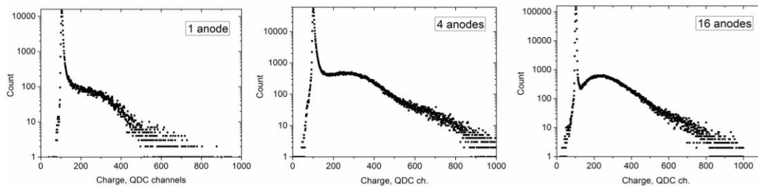
Figure 3. Single photoelectron amplitude spectra measured by 1, 4 and 16 interconnected anodes.
