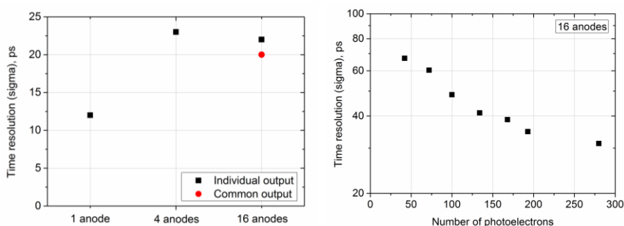
Figure 5. Summary of the time resolution measurements under the detection of 100 photoelectrons light pulses with different number of interconnected anodes for individual and common outputs. The measurements were carried out with LeCroy WR 620Zi digital oscilloscope.
