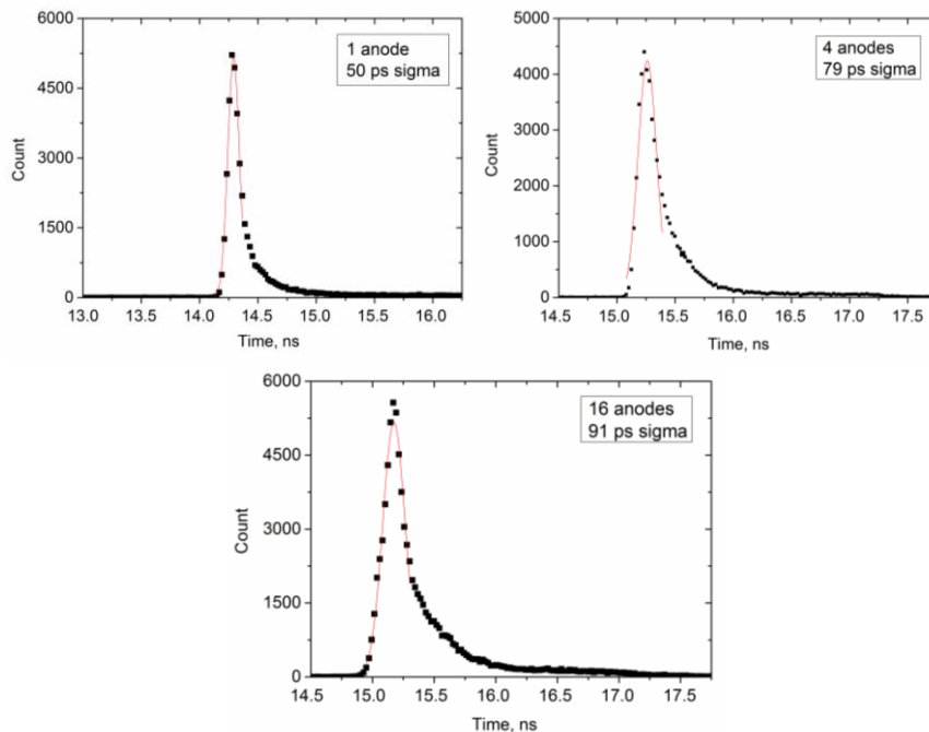
Figure 4. Time distribution spectra for single photon light pulses measured by 1, 4 and 16 interconnected anodes.
