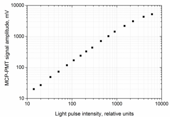
Figure 2. Dependence of the PMT signal amplitude (detected by 16 anodes) on the laser pulses' intensity ( U_b = 1300 V, A_{MIP} = 50 mV).
