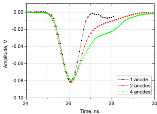
Figure 1. Signal waveforms from different number of the PMT anodes (1, 2 and 4), interconnected electrically.
