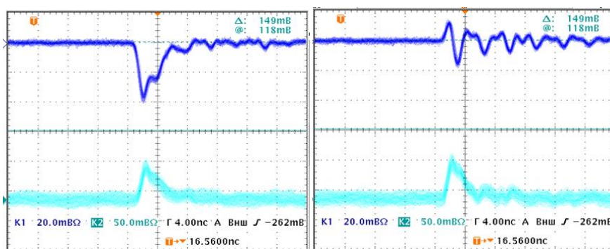
Figure 7. Waveform curves from 16 interconnected individual outputs (top curves) and from the common output (bottom curves). Please, refer to the text above for more detailed description.
