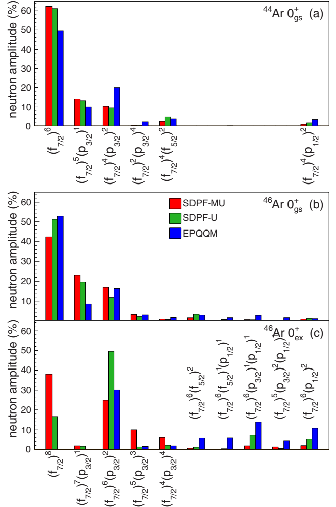
FIG. 12. Calculated wave functions of the ground state of ^{44}\text{Ar} (a) and two 0^+ states in ^{46}\text{Ar} , (b) for the ground state, and (c) for the first excited 0^+ state. Only the largest neutron components are shown.
