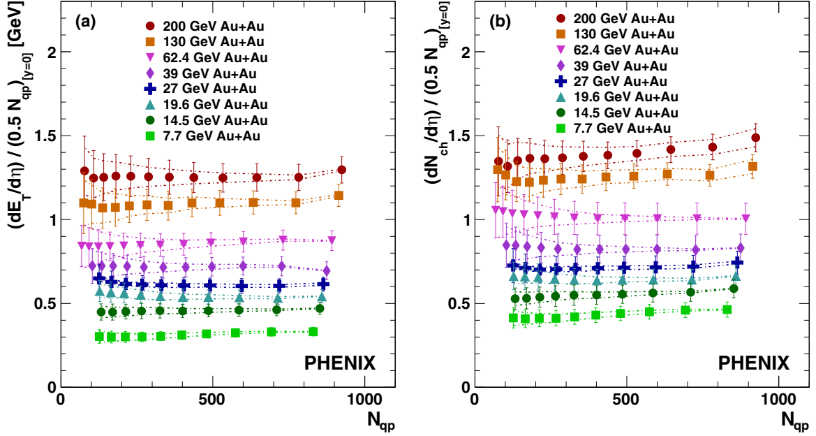
FIG. 16. (dE_T/d\eta)/(0.5N_{qp}) (a) and (dN_{ch}/d\eta)/(0.5N_{qp}) (b) at midrapidity as a function of N_{qp} for Au + Au collisions at \sqrt{s_{NN}} = 200, 130, 62.4, 39, 27, 19.6, 14.5, and 7.7 GeV. The lines bounding the points represent the trigger efficiency uncertainty within which the points can be tilted. The error bars represent the remaining total statistical and systematic uncertainty.
