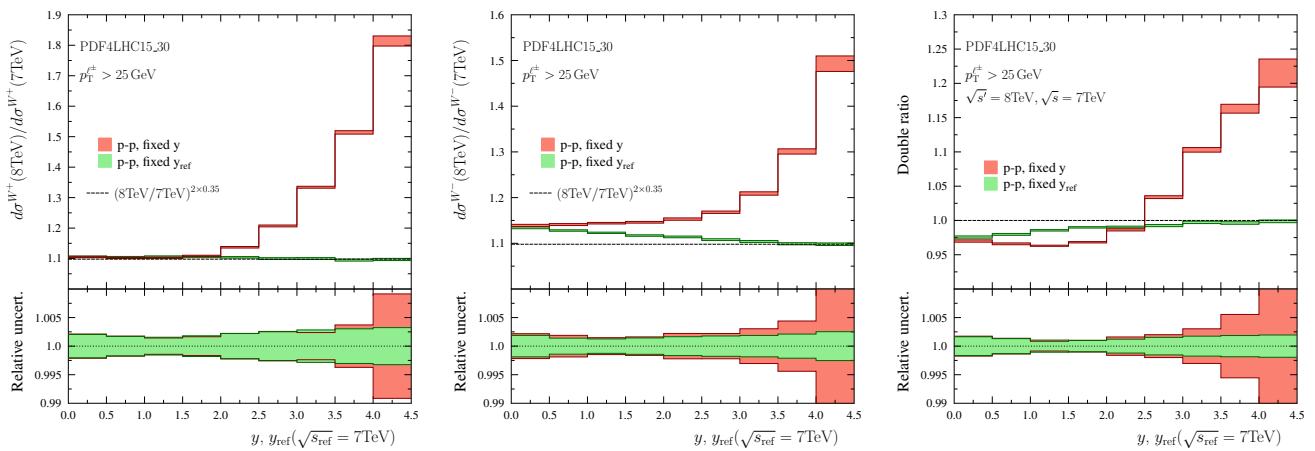
Fig. 7 Ratios of l^+ (left) and l^- (middle) spectra computed at \sqrt{s} = 8 TeV and \sqrt{s} = 7 TeV centre-of-mass energies. In red color are the results binned in lepton rapidity y , and in green the results binned in y_{\text{ref}} taking \sqrt{s_{\text{ref}}} = 7 TeV. The dashed lines indicate the prediction of scaling law Eq. (12). The right-hand panel shows the double ratio of Eq. (27)
