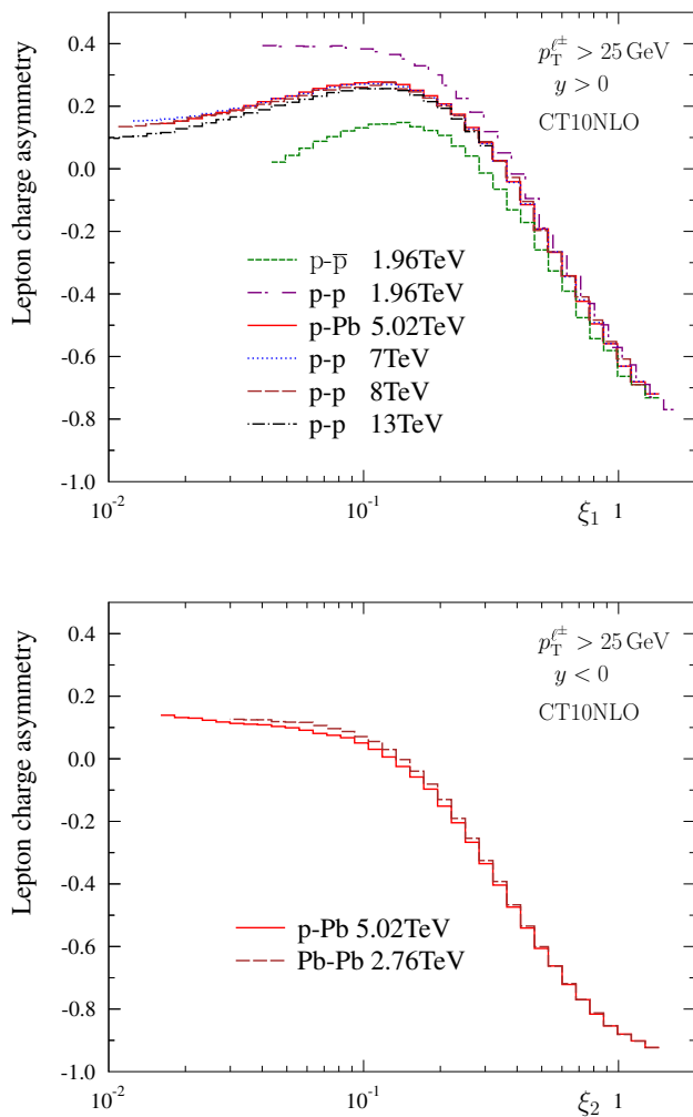
Fig. 3 Lepton charge asymmetry in p-p̄ ( \sqrt{s} = 1.96 TeV), p-p ( \sqrt{s} = 1.96, 7, 8 TeV), p-Pb ( \sqrt{s} = 5.02 TeV) and Pb-Pb ( \sqrt{s} = 2.76 TeV) collisions, for y > 0 (upper panel) and y < 0 (lower panel)
