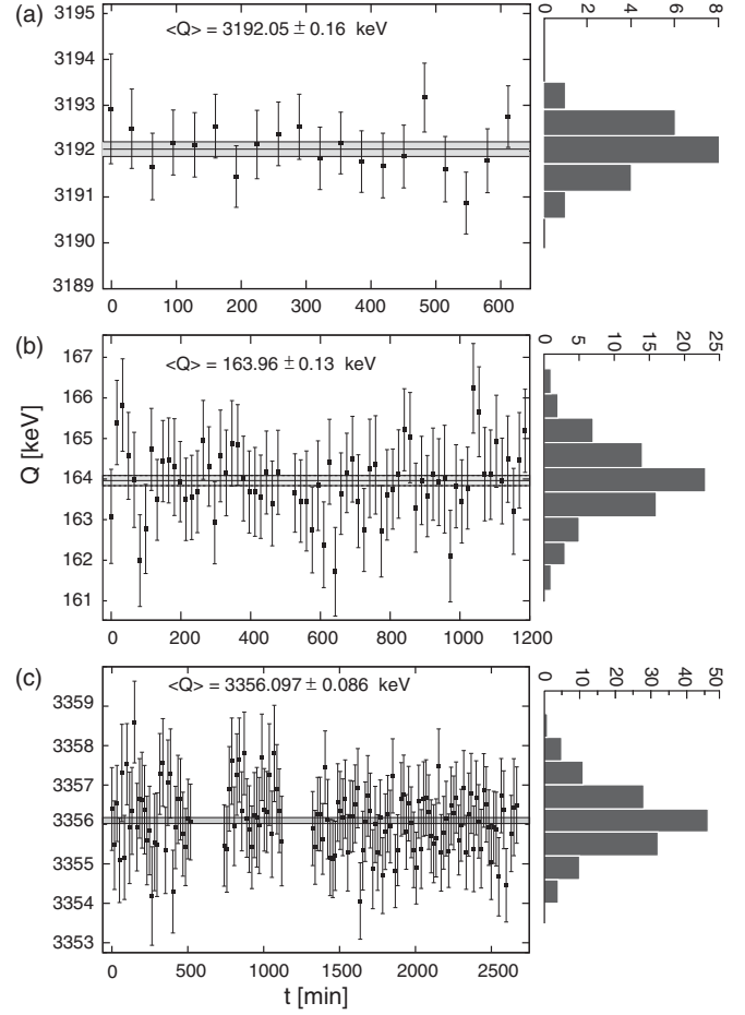
FIG. 3. Q -value results for (a) ^{96}\text{Nb} to ^{96}\text{Mo} , (b) ^{96}\text{Zr} to ^{96}\text{Nb} , and (c) ^{96}\text{Zr} to ^{96}\text{Mo} decays. The individual measurements are plotted against the elapsed time of the experiment. The grey bands indicate the final errors around the central values. Also shown is the distribution of the individual measurements within \pm 300 eV bins indicating a normal distribution.
