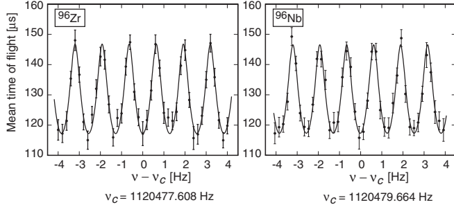
FIG. 2. Time-of-flight spectrum for the ( ^{96}\text{Zr}, ^{96}\text{Nb} ) pair using a 25-750-25 ms (on-off-on) Ramsey excitation pattern. The solid line represents a fit to the data using the theoretical line shape as described in Ref. [26].
