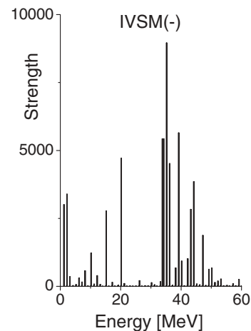
FIG. 4. Results of the realistic calculation for the IVSM^- strength. IVSM^- transitions have been calculated by including all possible \Delta N = 0, 2 contributions.
