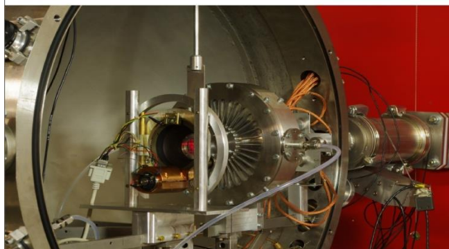
Figure 4. Reaction chamber with rotating target and gas catcher.
