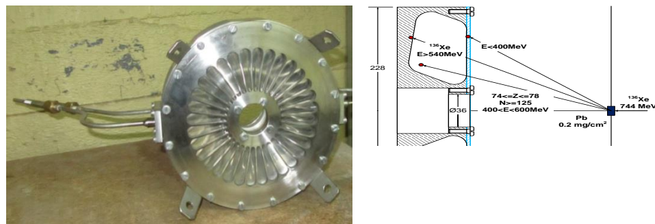
Figure 3. Gas catcher
