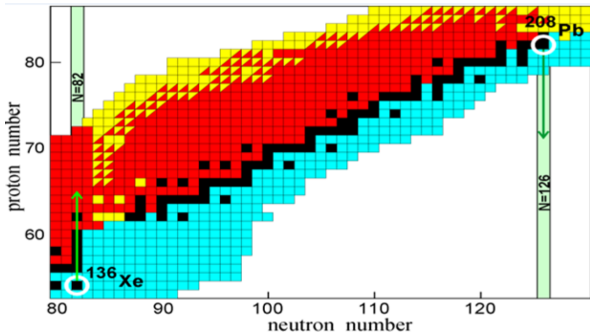
Figure 1. Chart of nuclide demonstrates possibility of proton transfer in reaction of ^{136}\text{Xe}+^{208}\text{Pb} at energy near Coulomb barrier (black squares – stable nuclei).[1]
