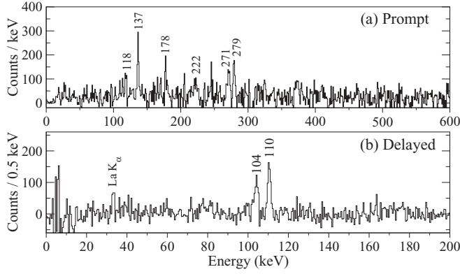
FIG. 10. Spectra produced from a prompt-delayed \gamma - \gamma coincidence matrix for ^{130}\text{La} . The matrix had an optimum recoil-delayed \gamma correlation time of 2.5\ \mu\text{s} and was background subtracted. (a) Prompt \gamma rays that correlate with delayed 110 keV decays. (b) Delayed \gamma rays that correlate with prompt 137 keV decays.
