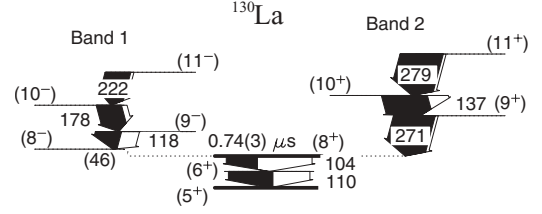
FIG. 12. Partial ^{130}\text{La} decay scheme produced in this work. The newly observed delayed \gamma rays at 104 and 110 keV are tentatively positioned below the proposed (8^+) isomeric state. The weighted mean of the half-lives measured from the 104 and 110 decay time distributions is adopted as the half-life for the (8^+) state. The 46 keV decay was reported in a previous study [12] but not observed in this work.
