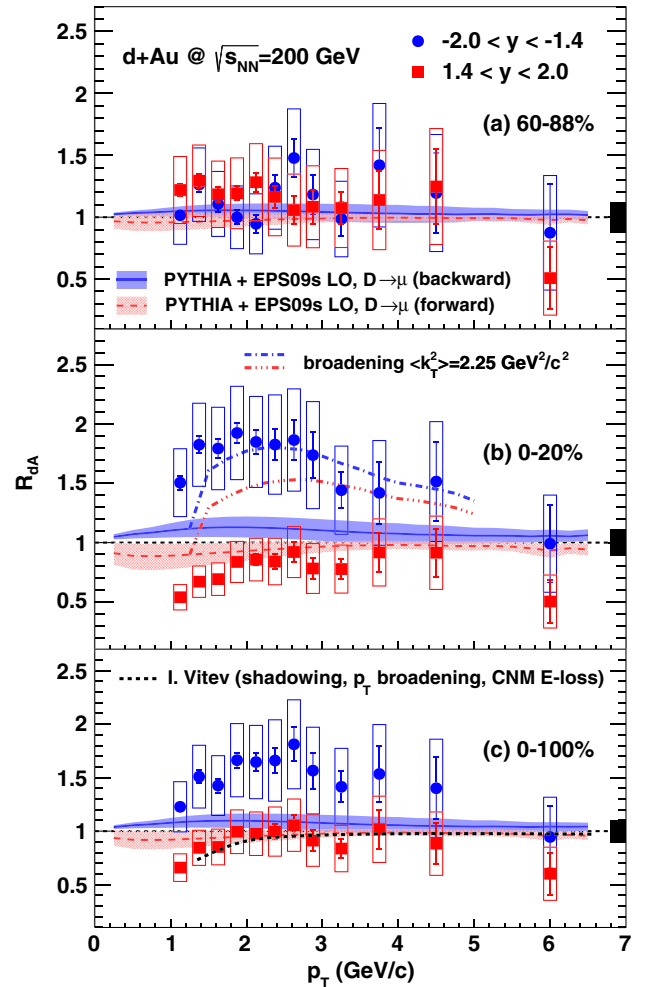
FIG. 2 (color online). The nuclear modification factor R_{dA} for negatively charged heavy-flavor muons in d+Au collisions for the (a) most peripheral (60%–88%) and (b) most central (0%–20%) centrality classes, and (c) unbiased (0%–100%) data. The black boxes on the right side indicate the global scaling uncertainty. The red dashed (blue solid) lines in each panel are calculations at forward (backward) rapidity based on the EPS09s nPDF set [14]. Dot-dashed curves in (b) are the same calculations plus an additional nuclear- p_T broadening. The theoretical calculation shown in (c) is for forward rapidity [16].
