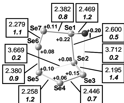
Conformation 10_1 (0.0 kJ mol -1 )
