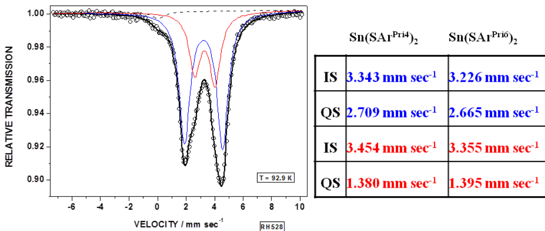
Figure 7. Mössbauer spectrum for \text{Sn}(\text{SAr}^{\text{Pri}_4})_2 ( 9 ) at 93 K, with tabular data for
