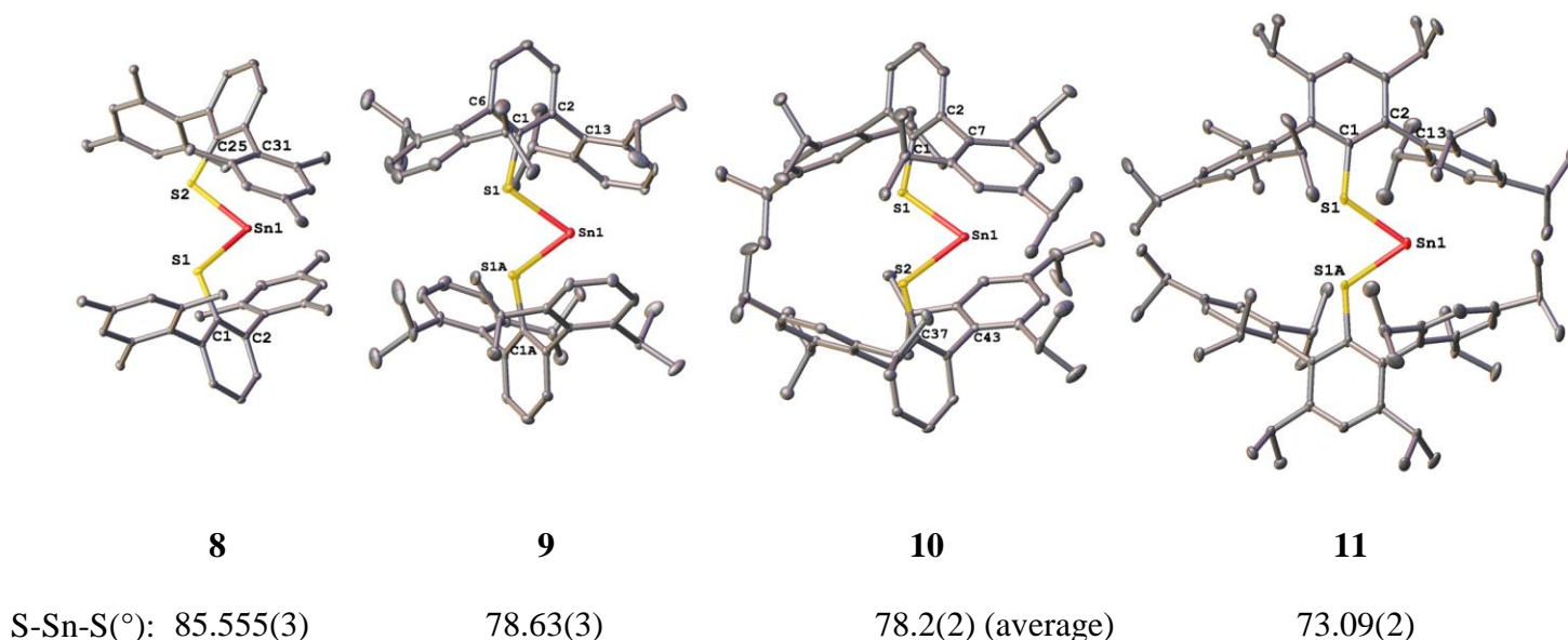
Figure 2. X-ray structures of tin dithiolates 8-11 (30% probability ellipsoids) without hydrogen atoms, for the Sn(II) derivatives of the SAr Me 6 , SAr Pri 4 , SAr Pri 6 , and SAr Pri 8
