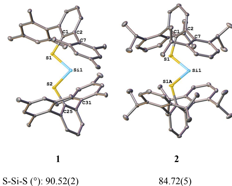
Figure 3. Thermal ellipsoid plot (30 %) of the structures of 1 and 2 (30 % probability ellipsoids); hydrogens are not shown for clarity. 2 features the narrowest R-Si-R angle ( 84.72(5)^\circ ) for a two-coordinate silylene (cyclic or acyclic).
