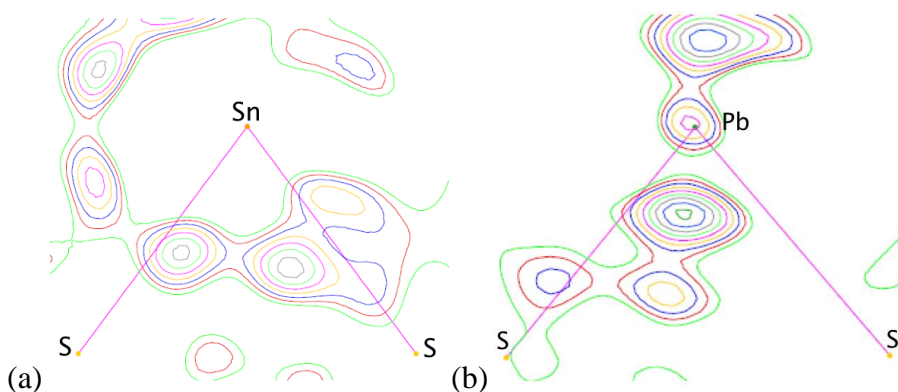
Figure 10. Difference electron density map of (a) \text{Sn}(\text{SAr}^{\text{Pri}8})_2 ( 11 ) shows contours of electron density bisecting the two M-S bonds. (b) \text{Pb}(\text{SAr}^{\text{Pri}8})_2 ( 14 ) shows a buildup of electron density within the S-Pb-S plane. Lines are shown connecting the sulfur and lead nuclei.
