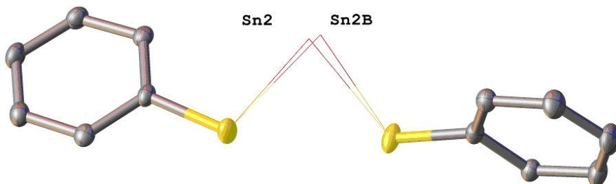
Figure 6. X-ray crystal structure of one of the molecules of \text{Sn}(\text{SAr}^{\text{Pri}6})_2 in the asymmetric unit. For clarity, flanking arene rings are not shown.
