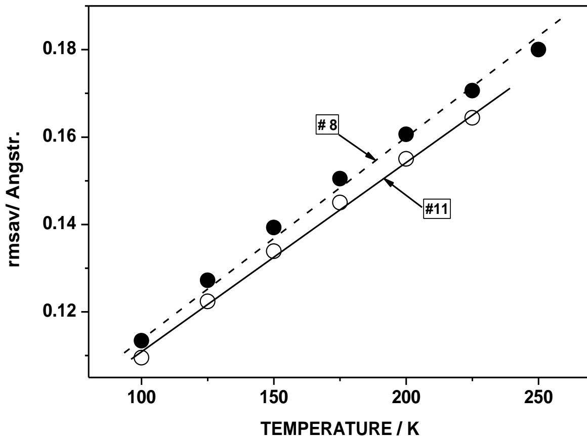
Figure 8. The root-mean-square-amplitude-of-vibration of the Sn atoms in two of the compounds discussed in the text, calculated from the temperature-dependent ^{119}\text{Sn} Mössbauer data.
