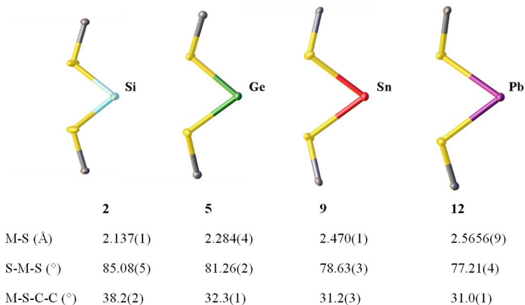
Figure 4. Drawings of the core atoms in the bithiolato tetrylenes M(\text{SAr}^{\text{Pri}4})_2 ( M = \text{Si} , 2 ; \text{Ge} , 5 ; \text{Sn} , 9 ; \text{Pb} , 12 ). (30% probability ellipsoids) derivatives with identical \text{SAr}^{\text{Pri}4} ligands showing that the S-M-S angle becomes narrower with increasing atomic number.
