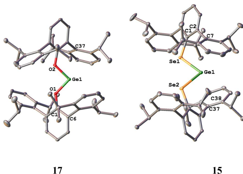
Figure 5. X-ray structures of the bisphenoxo and bis-selenolato germylenes 17 and 15 (30% probability ellipsoids) without hydrogen atoms. The O1-Ge1-O2 = 92.54(6)°; Se1-Ge1-Se2 = 84.75(1)°. Other structural data are given in Table 4.
