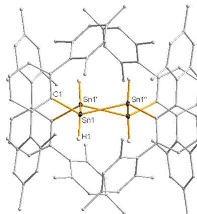
Figure 2. X-ray crystal structure of 2 ·2Et 2 O. Solvent molecule and aryl hydrogen atoms are not shown for clarity. Thermal ellipsoids are drawn with 30 % probability. Selected bond lengths (Å) and angles (°): Sn(1)-Sn(1'): 2.8433(4), Sn(1)-Sn(1''): 2.8050(3), Sn(1)-C(1): 2.173(3), Sn(1)-H(1): 1.47(5), C(1)-Sn(1)-Sn(1'): 130.89(7), Sn(1)-Sn(1')-Sn(1''): 87.030(3).
