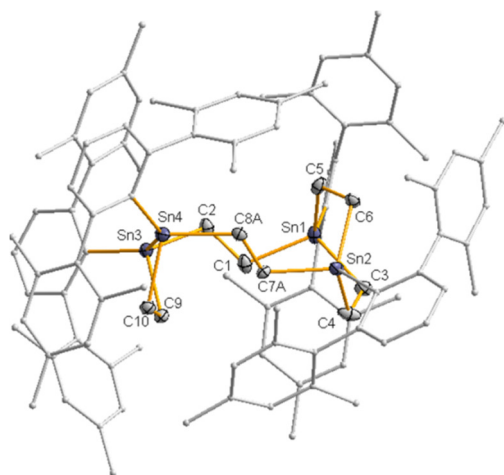
Figure 1. X-ray crystal structure of 1 ·2Et 2 O. One of the disordered ethylene (C7B-C8B) positions, solvent molecules and hydrogen atoms are not shown for clarity. Thermal ellipsoids are drawn with 30 % probability. Selected bond lengths (Å) and angles (°): Sn(3)-Sn(4): 2.8549(5) Sn(1)-C(1): 2.181(4) C(1)-C(2): 1.538(6) Sn(3)-C(9): 2.208(4) Sn(3)-C(59): 2.205(4), C(1)-Sn(1)-C(3): 108.82(17), C(1)-Sn(1)-C(5): 106.15(17), C(2)-Sn(3)-C(9): 110.36(16).
