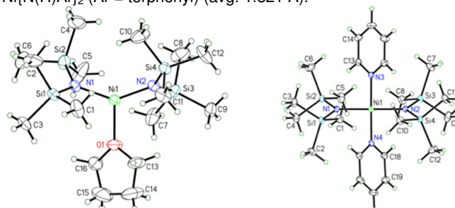
Figure 1. Thermal ellipsoid (50%) plots of Ni{N(SiMe 3 ) 2 } 2 (THF) ( 2 , left) and Ni{N(SiMe 3 ) 2 } 2 (py) 2 ( 3 , right). Selected bond lengths (Å) and angles (°) for 2 : Ni1-N1 1.8646(2), Ni1-N2 1.8570(2),
