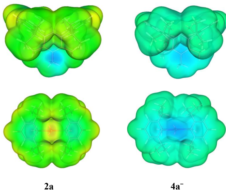
Figure 4. Molecular electrostatic potentials for 2a and 4a - . For clarity, the potentials are shown in direction perpendicular to the C 2 B 2 N 2 ring (above) and along the transannular C...C axis of the C 2 B 2 N 2 ring (below). Color code: blue (negative) – turquoise – green (neutral) – yellow – orange (positive).
