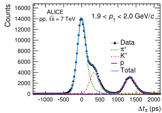
Fig. 4 Distribution of \Delta t_i assuming the pion mass hypothesis in the transverse momentum interval 1.9 < p_T < 2.0 \text{ GeV}/c . The data (black points) are fitted with a function (light blue line) that is the sum of the signal due to pions (green dotted line) and the two populations corresponding to kaons (red dotted line) and protons (purple dashed line)
