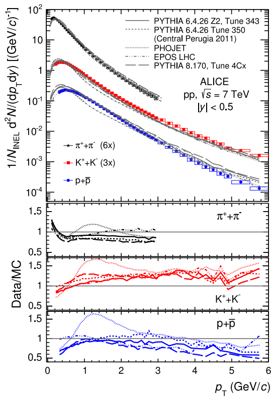
Fig. 18 Top panel measured p_T spectra of pions, kaons and protons, sum of particles and antiparticles, compared to PYTHIA6-Z2, PYTHIA6-CentralPerugia2011, PYTHIA8, EPOS LHC and PHOJET Monte-Carlo calculations. Statistical (vertical error bars) and systematic (open boxes) uncertainties are reported for the measured spectra. Bottom panels ratios between data and Monte-Carlo calculations
