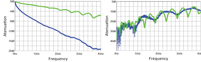
Figure 6.13: 4 m Samtec Twinax insertion loss (left) and return loss (right). The green line represents the contribution of the measurement system reference (which was characterised on purpose); the blue line the cable plus the test system.
