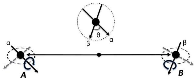
Figure 1. Entanglement paradigm. Schematic representation of two spin-1/2 particles, e.g., electrons, in the singlet state (represented by \langle \uparrow \downarrow | \otimes \langle \downarrow \uparrow | - | \downarrow \downarrow \rangle \otimes | \uparrow \uparrow \rangle in quantum-mechanical notation) running away from each other. The directions \alpha and \beta are detector settings for spin measurements (in our language, inputs). The measured spins A and B (outputs) in these directions are shown by rotation arrows: one direction of rotation (say, clockwise) represents “spin-up” = +1 in one particle and “spin-down” = -1 in the other. By the quantum theory, for any \alpha, \beta , \Pr[A = +1, B = +1] = 1/2 \cos^2 \theta/2 (equivalently, expected value of AB is \cos \theta ). The two measurements are made simultaneously (in some inertial frame of reference). doi:10.1371/journal.pone.0061712.g001
