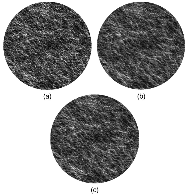
Fig. 4 (a) An image of a numerically generated (by deposition) network of fibers. (b) A coarse-grained version of this image with smoothing. (c) A coarse-grained version of this image without smoothing.
