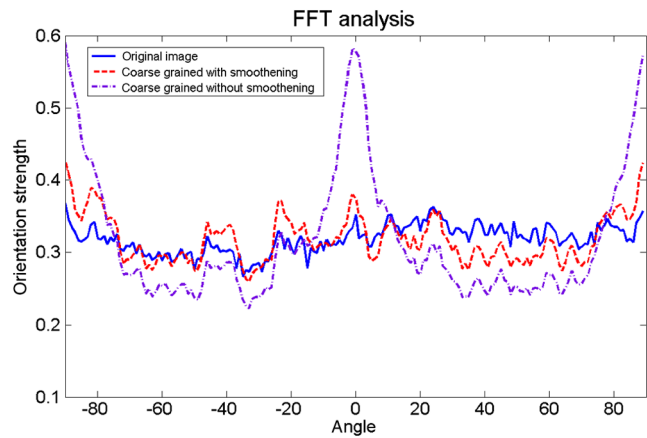
Fig. 13 FFT-based estimates for the distribution of fiber orientation of the original newsprint sample [Fig. 5(a)] and its two coarse-grained versions.
