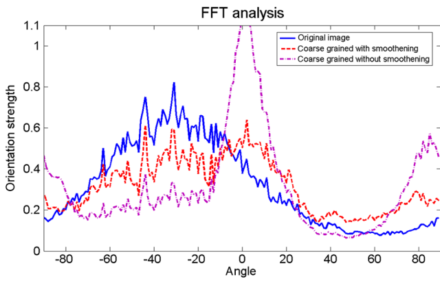
Fig. 10 FFT-based estimates for the distribution of fiber orientation as determined from the original generated network of Fig. 4(a) and its two coarse-grained versions (as explained in the text).
