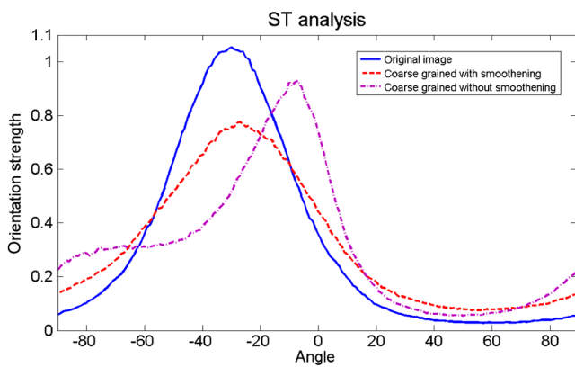
Fig. 11 ST-based estimates for the distribution of fiber orientation as determined from the original generated network of Fig. 4(a) and its two coarse-grained versions (as explained in the text).
