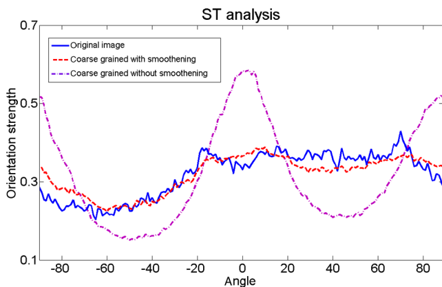
Fig. 17 ST-based estimates for the distribution of fiber orientation of the original nanofiber image [Fig. 6(a)] and its two coarse-grained versions.
