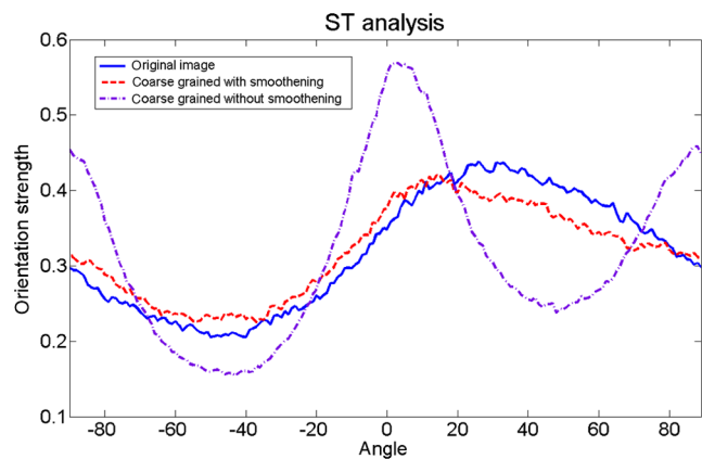
Fig. 14 ST-based estimates for the distribution of fiber orientation of the original newsprint sample [Fig. 5(a)] and its two coarse-grained versions.
