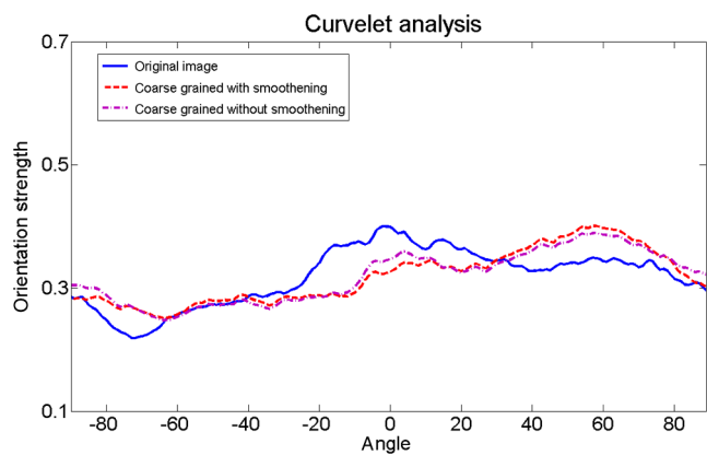
Fig. 15 Curvelet-based estimates for the distribution of fiber orientation of the original nanofiber image [Fig. 6(a)] and its two coarse-grained versions.
