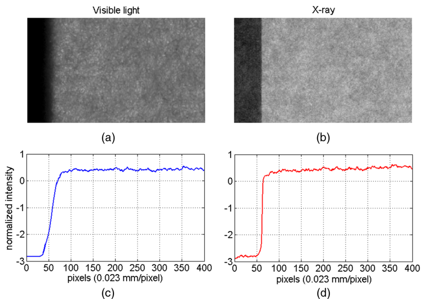
Fig. 2 Blurring of a sharp edge in the transmission of visible light (a) and x-rays (b) through paper. Normalized intensity of the transmission intensity of visible light (c) and x-rays (d).
