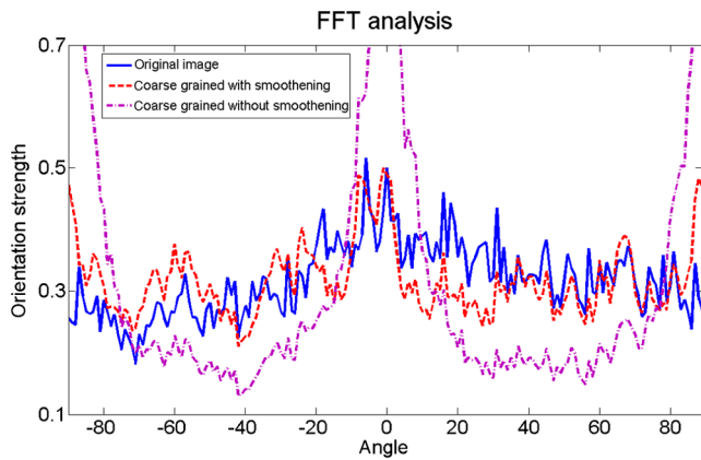
Fig. 16 FFT-based estimates for the distribution of fiber orientation of the original nanofiber image [Fig. 6(a)] and its two coarse-grained versions.
