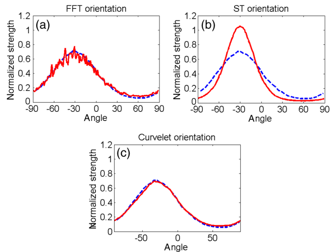
Fig. 8 Estimations for distribution of fiber orientation in the image of a numerically generated network of fibers shown in Fig. 4(a). Orientation distribution as determined by the FFT method (upper left panel), the one determined by the ST method (upper right panel), and the one determined by the curvelet method (lowest panel). Each panel includes also the known orientation distribution (the dashed lines) for comparison.
