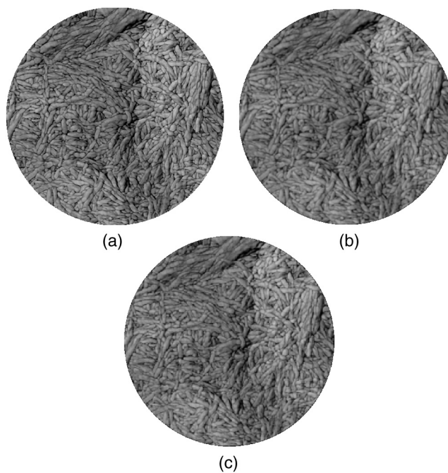
Fig. 6 An atomic force microscope image of a thin film made of organic nanofibrils. (b) A coarse-grained version of this image with smoothening. (c) A coarse-grained version of this image without smoothening.
