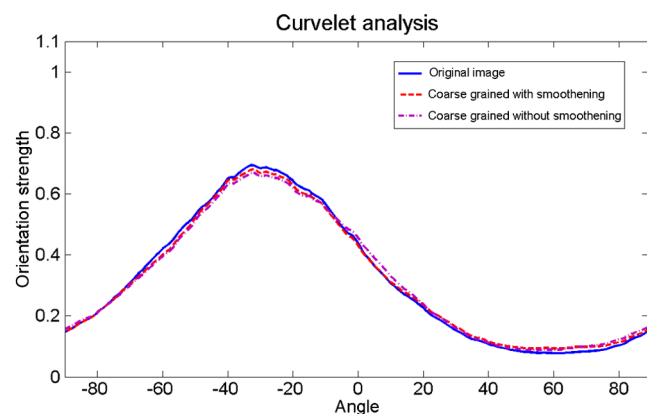
Fig. 9 Curvelet-based estimates for the distribution of fiber orientation as determined from the original generated network of Fig. 4(a) and its two coarse-grained versions (as explained in the text).
