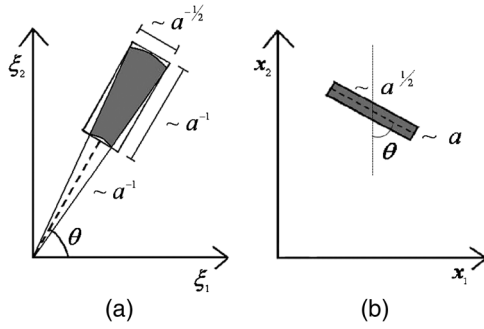
Fig. 3 Support of \hat{\gamma}_{ab\theta} in the frequency domain (a), and the area that contains most of the “energy” of \gamma_{ab\theta} (b).
