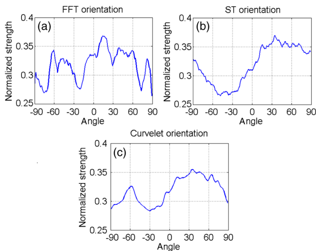
Fig. 7 Estimations for distribution of fiber orientation of the paper sample of Fig. 1. Orientation distribution determined by the fast Fourier transform (FFT) method (a), the one determined by the structure tensor (ST) method (b), and the one determined by the curvelet method (c).
