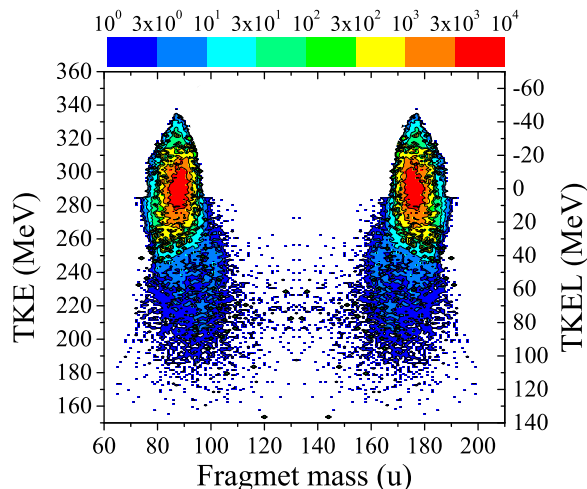
FIG. 2. (Color online) Mass-energy distribution of binary fragments obtained in the reaction ^{88}\text{Sr}+^{176}\text{Yb} at a c.m. energy of 290 MeV and integrated over the angular range of 45^\circ – 140^\circ in c.m. Only true two-body events are included (no sequential fission). On the right vertical axis the total kinetic energy lost (TKEL) scale is reported.
