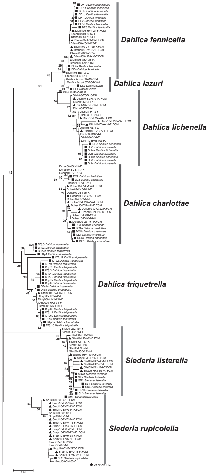
Fig. A5. Neighbour-joining phylogenetic tree based on K2P, pairwise deletion and bootstrap test of 500 replications for the seven species of bagworm moths. Bootstrap values are indicated next to each node. The phylogenetic tree includes a reference sequence of Narycia duplicella as an outgroup (black circles). Each sample name indicates the moth species: (Dlich = D. lichenella , Dlaz = D. lazuri , Dfenni = D. fennicella , Dtriq = D. triquetrella , Dchar = D. charlottae , Slist = S. listerella , Srupi = S. rupicolella ). The reference sequences (Grapputo et al. 2005) are indicated with black squares. The tree also includes individuals that were used for flow cytometry measurements (black triangles). The scale bar at the bottom of each tree indicates the percentage of bp differences.
