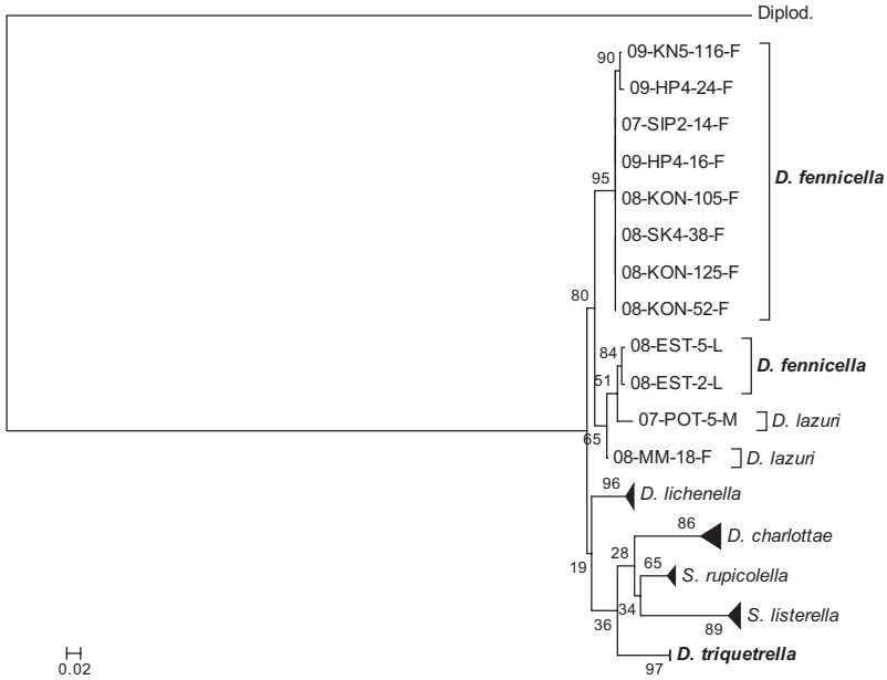
Fig. A2. Phylogeny of the genera Dahlica and Siederia based on a partial sequence of the nuclear gene MDH estimated by Maximum Likelihood (B) ( \text{Log}L = -2677.04697 ) according to the SYM + I + \Gamma model of nucleotide substitution. The bootstrap values are shown at the nodes of the tree. The outgroup is a sequence of D. laichartingella (Diplod). The parthenogenetic species are set in boldface. Some of the clusters ( D. triquetrella , D. lichenella , D. charlottae , S. rupicolella and S. listerella ) have been compressed in order to save space. The scale bar at the bottom of each tree indicates the percentage of bp differences.
