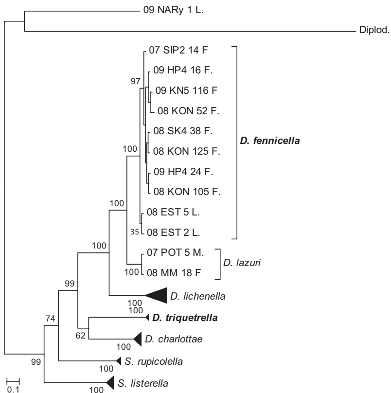
Fig. 4. Phylogeny of the genera Dahlica and Siederia based on the concatenated partial mitochondrial sequences estimated by Bayesian Inference according to the following models of nucleotide substitution: GTR + I ( COI ) HKY + I + \Gamma ( COII ). The Bayesian posterior probabilities are shown at the nodes of the tree. The outgroups are sequences of N. duplicella (09-NARY-1-L) and D. laichartingella (Diplod.). The parthenogenetic species are set in boldface. Some of the clusters ( D. triquetrella , D. lichenella , D. charlottae , S. rupicolella and S. listerella ) have been compressed in order to save space. The scale bar at the bottom of each tree indicates the percentage of bp differences.
