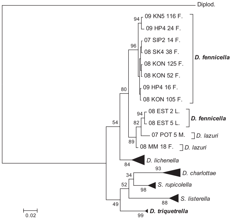
Fig. 3. Phylogeny of the genera Dahlica and Siederia based on a partial sequence of the nuclear MDH gene estimated by Bayesian Inference according to the SYM + I + \Gamma model of nucleotide substitution. The Bayesian posterior probabilities are shown at the nodes of the tree. The outgroup is a sequence of D. laichartingella (Diplod). The parthenogenetic species are set in boldface. Some of the clusters ( D. triquetrella , D. lichenella , D. charlottae , S. rupicolella and S. listerella ) have been compressed in order to save space. The scale bar at the bottom of each tree indicates the percentage of bp differences.
