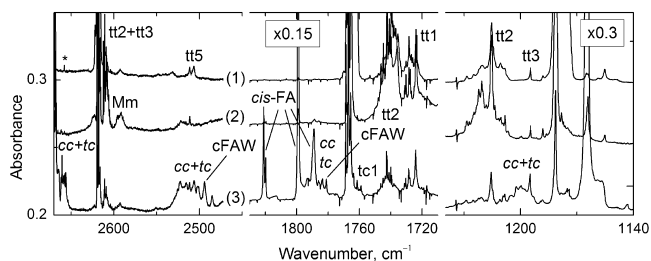
Figure 2. OD, C=O, and C–O stretching bands of HCOOD in an argon matrix. Shown are the results of deposition [trace 1], annealing at 34 K of matrices containing trans-FA [trace 2] and cis-FA [trace 3]. Mm marks the band of higher HCOOD multimers, cc and tc denote various cis–cis and trans–cis dimers, cFAW stands for the cis-HCOOD...D 2 O complex. The spectra were measured at 4.3 K. Water impurity (D 2 O) band is marked with asterisk.
