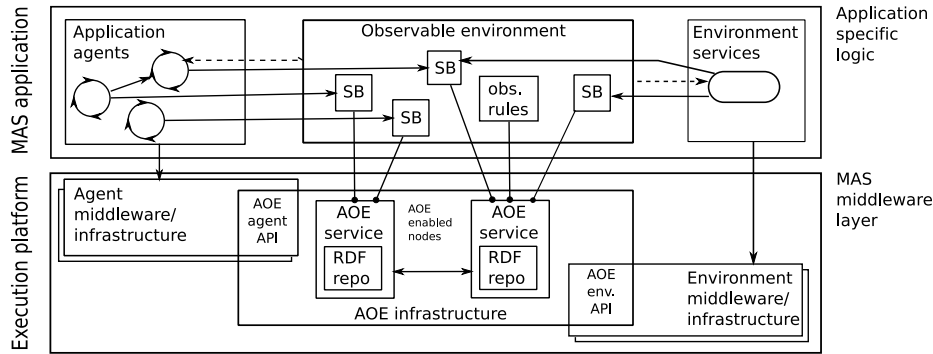
Figure 1. AOE logical architecture
