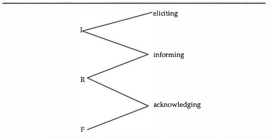
FIGURE 2.4 I-R-F Moves
