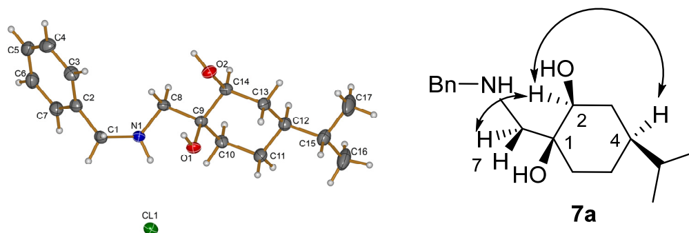
Figure 1. Structural determination of aminodiols 7a by X-ray crystallography and NOESY experiments.
