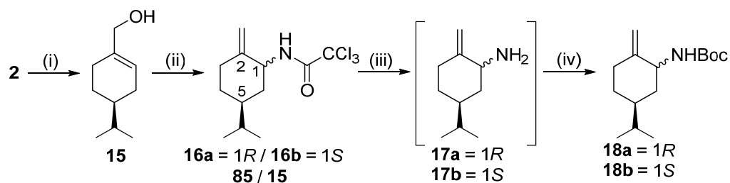
Scheme 4. Synthesis of the regioisomer allylamines via Overman rearrangement: (i) \text{NaBH}_4 , MeOH, 0 °C to rt, 1 h, 95%; (ii) (1) \text{CCl}_3\text{CN} , dry DCM, DBU, Ar atm, 0 °C to rt, 2 h; (2) toluene, Ar atm, 130 °C, 24 h, 72%, de = 70% for 16a ; (iii) (1) 5M NaOH/ \text{H}_2\text{O} , EtOH/DCM 2/1, 50 °C, 15 h; (iv) \text{Boc}_2\text{O} , cat. DMAP, THF, TEA, rt, 12 h, 59%.
