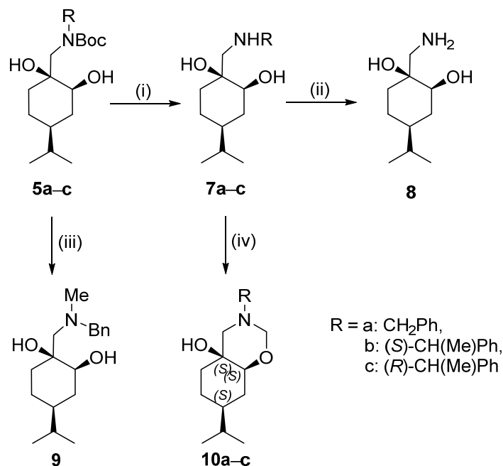
Scheme 2. Preparation of aminodiols starting from 5a–c : (i) Et 2 O, 18% HCl, overnight,, 82–88%; (ii) 10% Pd/C, n -hexane/EtOAc 1:2 mixture, 1 atm, H 2 , rt, 5 h, 35%; (iii) R = Bn, 3 eq. LiAlH 4 , THF, reflux, 6 h, 60%; (iv) 35% aq. CH 2 O, Et 2 O, rt, 3 h 70–96%.
