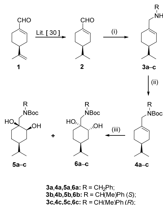
Scheme 1. Synthesis of BOC-protected aminodiols. (i) (1) 1.05 eq. R-NH 2 (R = a: CH 2 Ph, b: CH(Me)Ph ( S ), c: CH(Me)( R )), dry EtOH, rt, 2 h; (2) 3 eq. NaBH 4 , dry EtOH, rt, 2 h, 66–86%; (ii) Boc 2 O, TEA, DMAP, THF; rt, 90–95%; (iii) 50% NMO/H 2 O, cat. 2% OsO 4 in tert -BuOH, acetone/H 2 O, rt, 2 h, 25–48%, 5:6 = 1:1.
