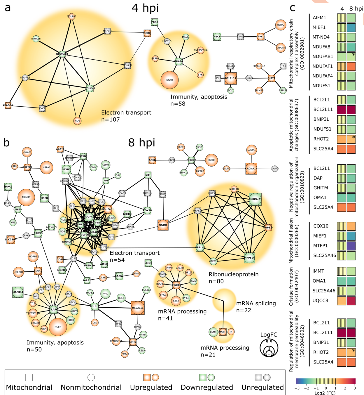
Fig 1. HSV-1 infection alters the host transcriptome. Global run-on sequencing (GRO-seq) analysis of nascent RNA levels of mitochondrial and mitochondria-associated proteins in infected Vero cells at (a) 4 and (b) 8 hpi. The genes encoding for mitochondrial proteins (square-shaped nodes, bolded titles) and nonmitochondrial cellular interactor proteins (round-shaped nodes) are shown. The upregulated (orange) or downregulated (green) transcripts in response to infection are visible together with unregulated interacting transcripts (grey). The node size correlates with a logarithmic fold change (logFC) of regulation and the thickness of black lines between nodes is proportional to the interaction in the STRING database ( https://string-db.org/ ). The main functions of the proteins are denoted with yellow circles with their size proportional to the number of interactors. (c) GO term classification for mitochondrial processes in the infected cells at 4 and 8 hpi. The color bar indicates upregulation (orange-red) or downregulation (green-blue), and low change of gene transcription (vertical stripes). The non-significant enrichment is also shown (*).
