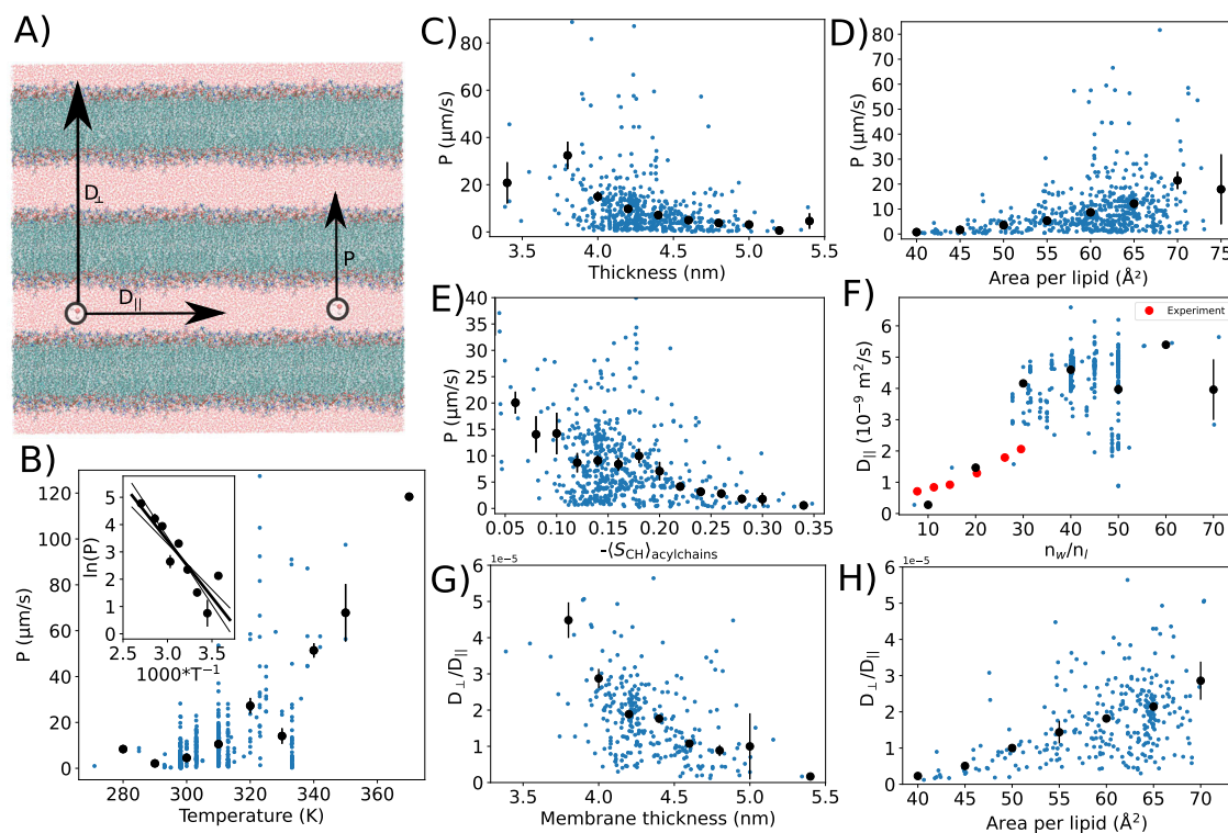
Fig. 5 | Quantification of water diffusion in NMRlipids Databank simulations. A Water diffusion, D_L , and permeability, P , through membranes, and lateral diffusion along the membrane, D_{||} , illustrated in a multilamellar stack of lipid bilayers. B–E Water permeation through membranes analyzed from the Databank as a function of temperature, thickness, area per lipid, and acyl chain order. Inset in (B) shows the Arrhenius plot of permeation ( \ln(P) vs. 1/T ) that gives 14 \pm 3 \text{ k}_B T for the average activation energy for water permeation through lipid bilayer. F Lateral diffusion of water as a function of hydration level. Experimental points for DMPC
