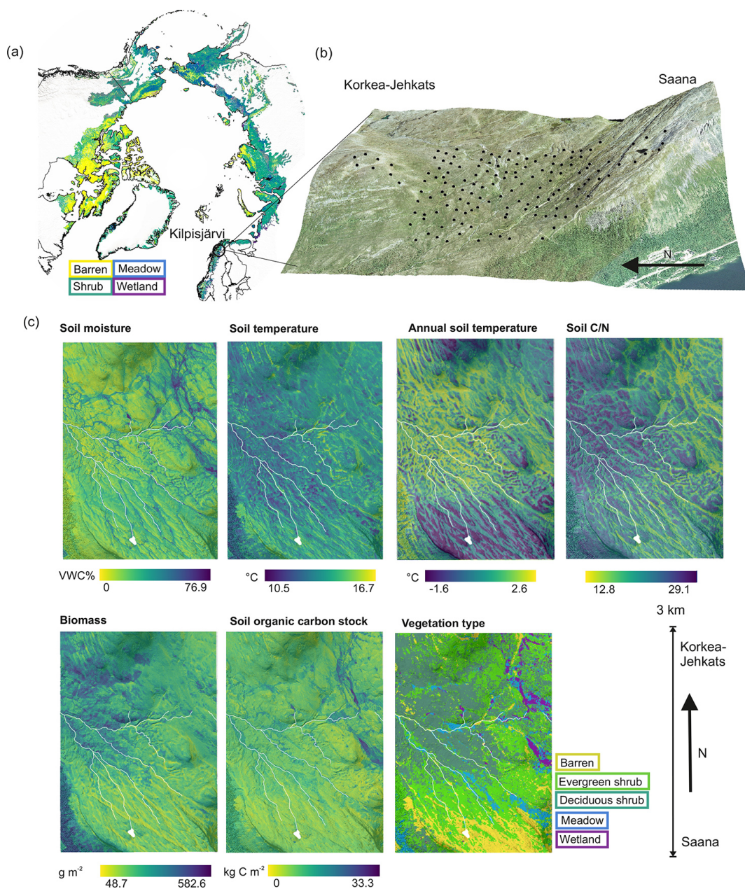
Figure 1. The distribution of the main vegetation types across the Arctic tundra (Dinerstein et al., 2017; European Space Agency, 2017) and the location of our study area (a), the distribution of plots (b) and environmental conditions derived from statistical upscaling of in situ measurements (see Sect. 2.3.2) across the study area (c). Soil moisture and temperature represent mean daytime (08:00 to 20:00 EET) conditions from 1 July to 2 August, and annual soil temperature is an average within the entire year (July 2017–June 2018). Other variables represent growing season conditions and are considered static in this study. The aerial image is produced by the National Land Survey of Finland (2016).
