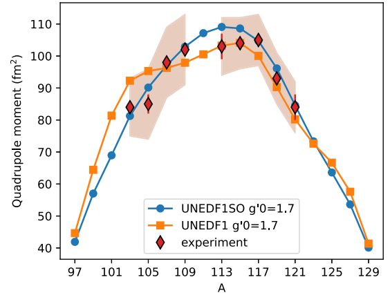
Fig. 4. Comparison of experimental and theoretical spectroscopic quadrupole moments of the 7/2^+ states. Colour code is the same as in Fig. 3. The red shaded area indicates the uncertainty due to the reference B/Q , while the error bars indicate only our statistical uncertainty on B .
