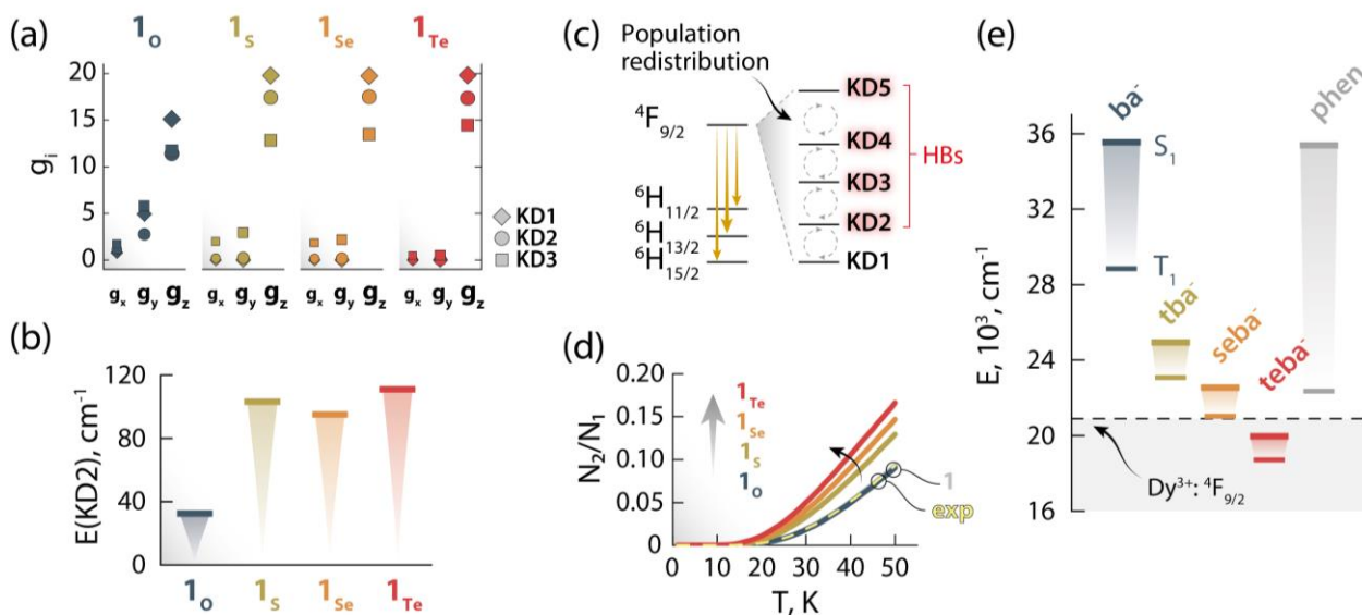
Figure 6. The effects of changing the chalcogen atom in the benzoate ligand on the magnetic and optical properties. Components of the g -tensor ( g_x , g_y , g_z ) of the first three KDs (a) and energy of KD2 (b) for the ground Dy^{3+}:^6H_{15/2} state of 1_o , 1_s , 1_{se} , and 1_{te} . Scheme depicting the temperature-induced electron population redistribution between the KDs (i.e., m_j levels) of the Dy^{3+}:^4F_{9/2} excited state (c). Ratio between the electron population of KD2 and KD1 as obtained from the Boltzmann model for 1_o , 1_s , 1_{se} , and 1_{te} (d). The results of the same calculations for 1 (solid gray line, beneath 1_o ) and considering the position of the ^4F_{9/2} components obtained from the deconvolution (Figure S11) of the ^6H_{15/2} \rightarrow ^4F_{9/2} transition in the excitation spectrum (exp, dashed yellow line) are also reported. The overlap between the curves 1 and 1_o is a serendipitous result stemming from the similar energy difference between the first two ^4F_{9/2} m_j levels obtained for these two systems. Energy of the first singlet ( S_1 ) and triplet ( T_1 ) excited states of the different ligands as obtained using the CAM-B3LYP exchange-correlation functional (e). The position of the Dy^{3+}:^4F_{9/2} excited state is also indicated with a dashed black line (centroid of the ^4F_{9/2} manifold obtained from the deconvolution of the ^6H_{15/2} \rightarrow ^4F_{9/2} transition in the excitation spectrum – Figure S10).
