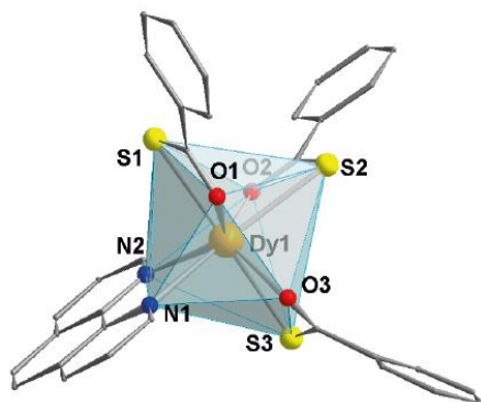
Figure 1. Partially labelled molecular structure of ( 1 ). Hydrogen atoms are omitted for clarity. Colour code: Dy – orange; O – red; S – yellow; N – blue.
