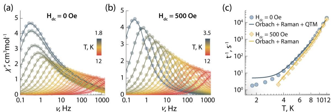
Figure 2. Frequency dependence of the out-of-phase ( \chi'' ) magnetic susceptibility as a function of temperature obtained in absence of an external dc magnetic field (a) and under an applied static field of 500 Oe (b). c) Temperature dependence of the magnetic relaxation times ( \tau ) in absence (blue circles) and in the presence of a 500 Oe applied field (yellow diamonds). Solid lines are the best fit to the experimental data using Eq. (1).
