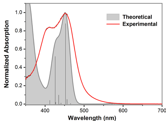
Figure 7. Experimental absorption spectrum of complex 4a in CH_3CN and the theoretical absorption spectrum convoluted with Gaussians of 30 nm width. The theoretical spectrum was shifted by 64 nm (0.45 eV) from 381 nm (3.25 eV) to 445 nm (2.80 eV) so that the maximum of the first absorption matches with the one observed experimentally.
