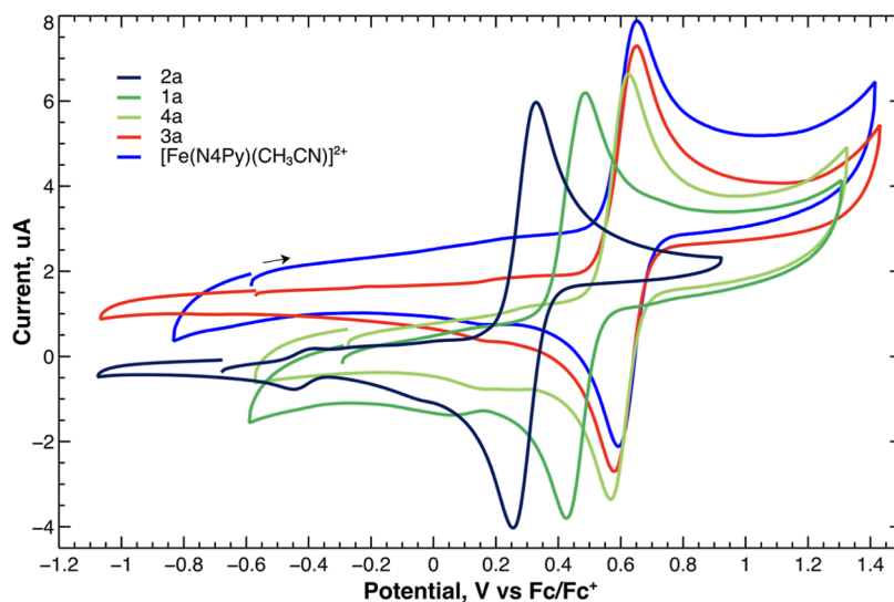
Figure 9. Cyclic voltammograms of 1\text{a} – 4\text{a} and [\text{Fe}(\text{N}4\text{Py})(\text{CH}_3\text{CN})]^{2+} in acetonitrile at 50 mV/s vs Fc/Fc + .
