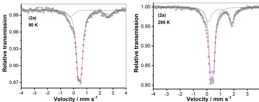
Figure 3. Zero-field Mössbauer spectra of the solid sample of complex 2a \cdot (\text{OTf})_2 at 80 K (left) and 295 K (right).
