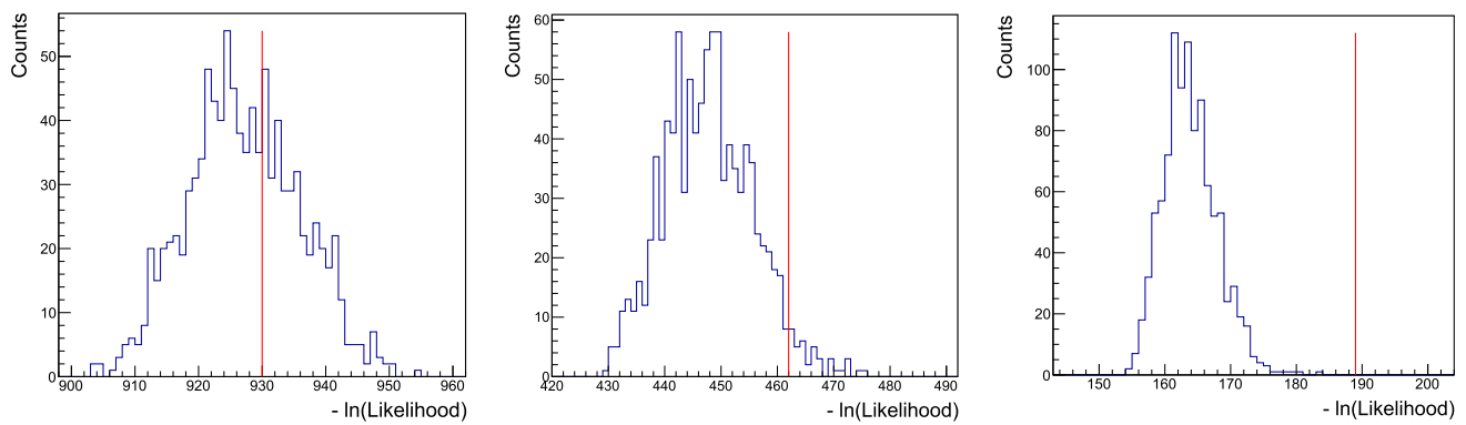
Fig. 10 Distribution of -\ln \mathcal{L}(\mathcal{D}|\vec{N}) from the toys for the \mathcal{M}_{1,\beta/\gamma} (left), \mathcal{M}_2 (middle) and \mathcal{M}_{1,\alpha} (right) spectra. The red line shows the -\ln \mathcal{L}(\mathcal{D}|\vec{N}) of the reference fit for each of the spectra
